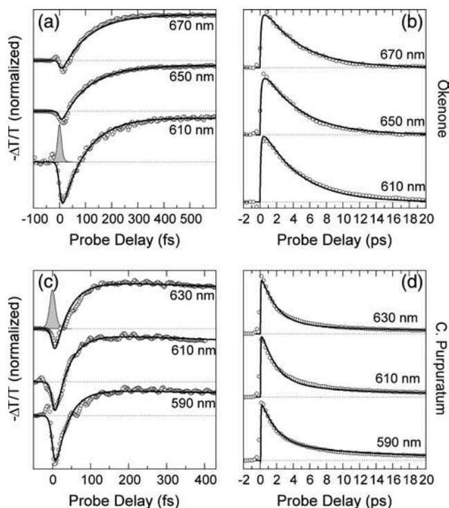
FIGURE 5 (Circles) \Delta T/T dynamics at different probe wavelengths of okenone in CS_2 (a and b) and the LH2 complex from C. purpuratum (c and d). Thick solid lines are fits obtained using the model described in the text. Pump-probe cross-correlation is shown as shaded area.
